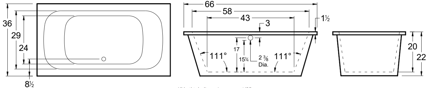
All bathtub dimensions are ± 1/2".
